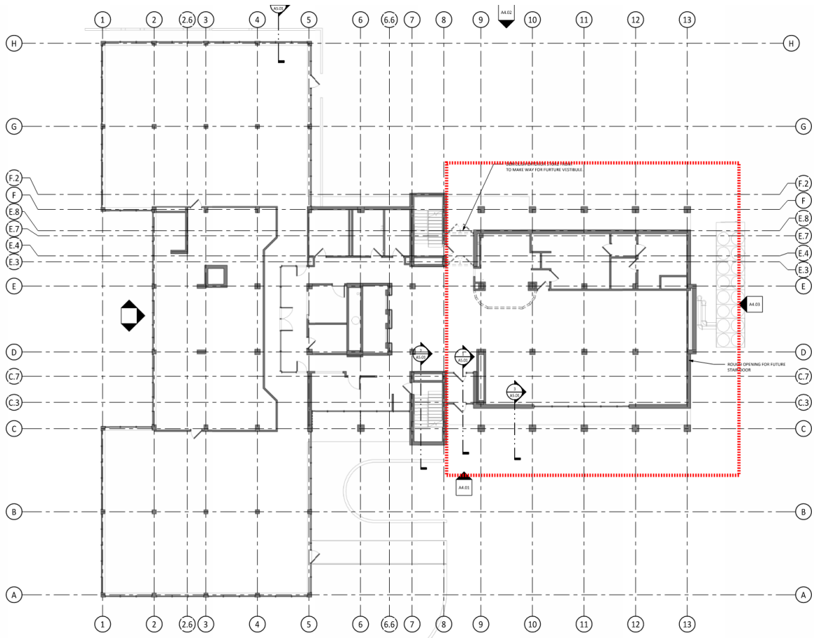
1 DEMO - LEVEL 1 SCALE 1/8" = 1'-0"
