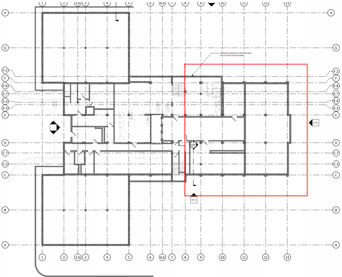
1 DEMO - LOWER LEVEL SCALE 1/8" = 1'-0"
