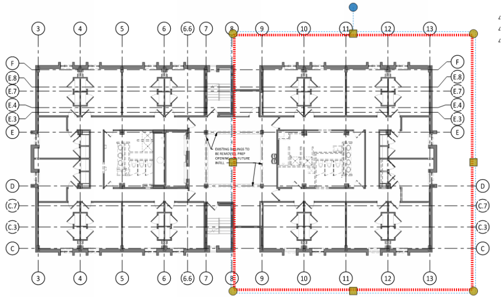
2 DEMO - LEVEL 3, 5, 7, & 9 SCALE | 1/8" = 1'-0"
